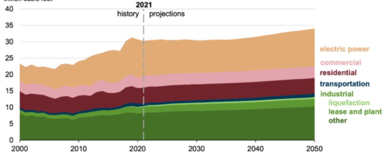
Natural gas consumption AEO2022 Reference case trillion cubic feet
