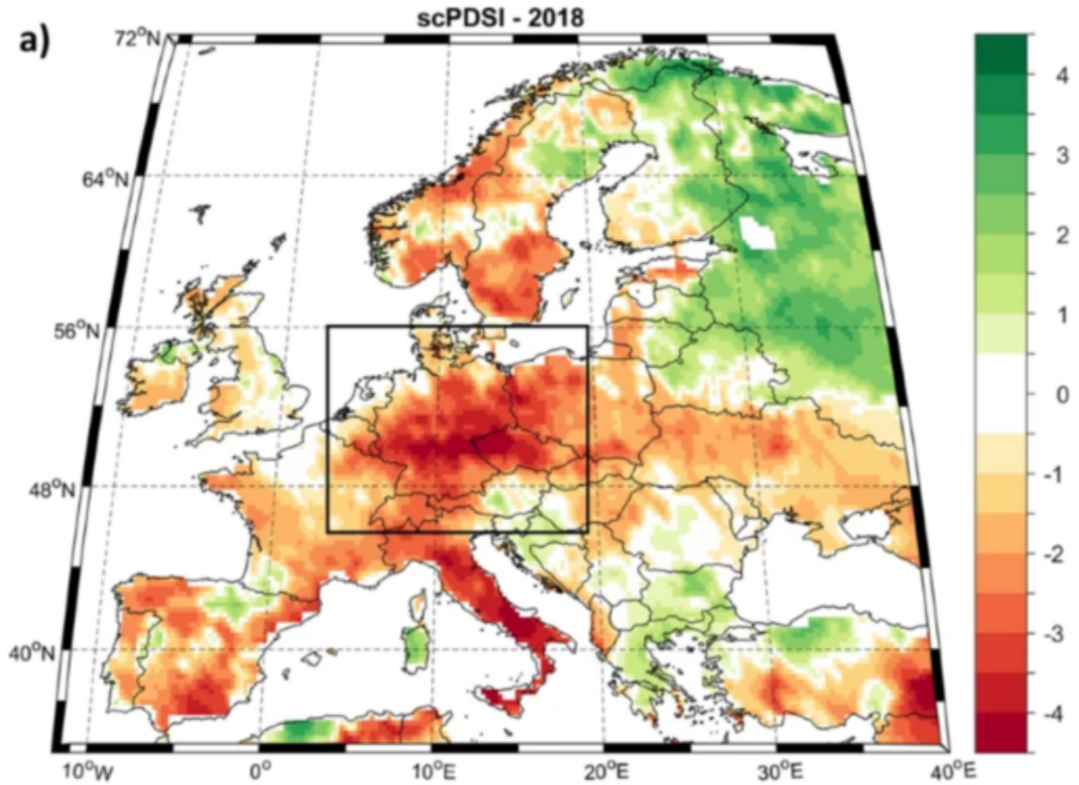
Fig. 1: Present-day drought variability.
