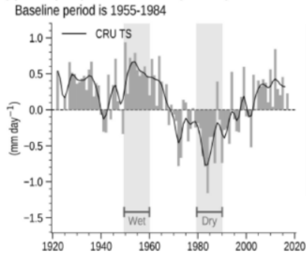
(a) Sahel precipitation anomalies (CRU TS)
