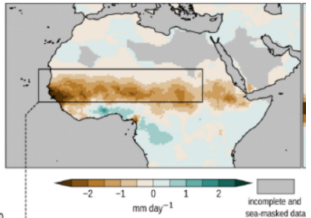
(b) Precipitation change over Africa CRU TS (1980-1990 – 1950-1960)
