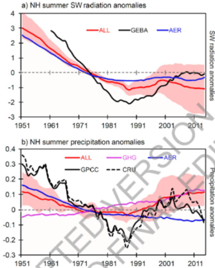
Box 8.1, Figure 1: Northern hemisphere surface downward radiation anomalies ( Wm^{-2} ; a) and precipitation anomalies ( mm/day ; b) for 1951–2014 for summer season (May–September) monsoon region (Polson et al. et al., 2014) from CMIP6 DAMIP experiments. Observed solar radiation anomalies are from GEBA global data from 1961–2014 (Wild et al., 2017) and observed precipitation anomalies are from GPCC and CRU. CMIP6 multi-model mean anomalies are from all-forcings (ALL), greenhouse gas forcing (GHG) and anthropogenic aerosol forcing (AER) experiments. Anomalies are with respect to 1961–1990 and smoothed with a 11-year running mean. Red shading shows the ensemble spread of ALL forcing experiment (5%–95% range). Models are masked to the GPCC data set. Further details on data sources and processing are available in the chapter data table (Table 8.SM.1).
