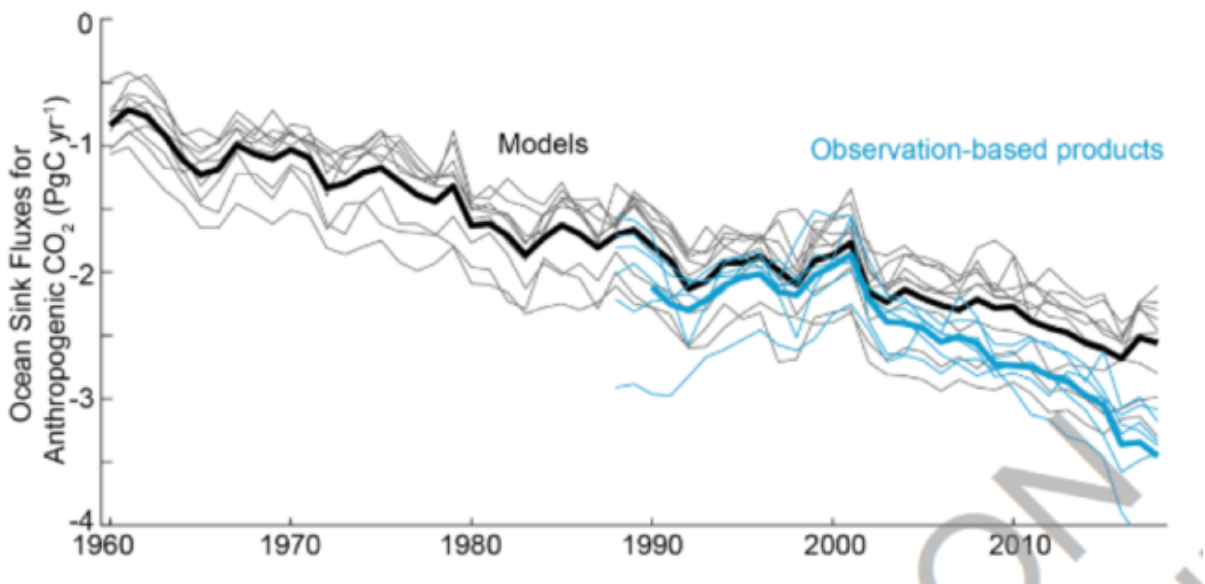
(a) Comparative trends in the ocean sink for anthropogenic CO 2 : models (1960–2018) and observation-based products (1987–2018)
