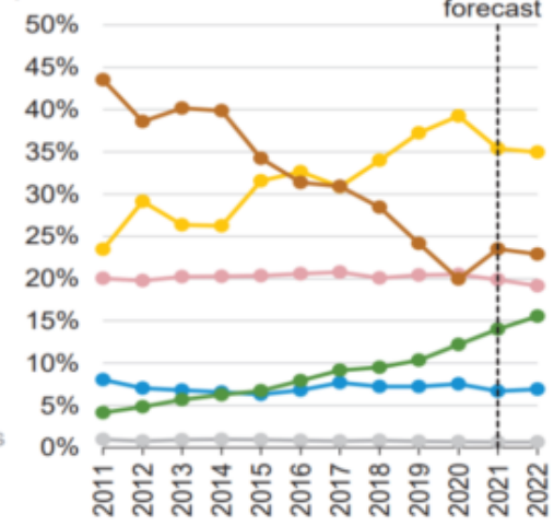
Source: U.S. Energy Information Administration, Short-Term Energy Outlook, May 2021
