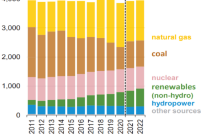
Source: U.S. Energy Information Administration, Short-Term Energy Outlook, May 2021
