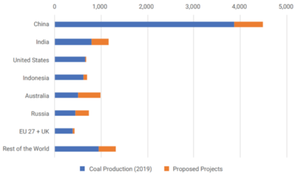
FIGURE 2: Proposed coal mines by country or region (mtpa)
