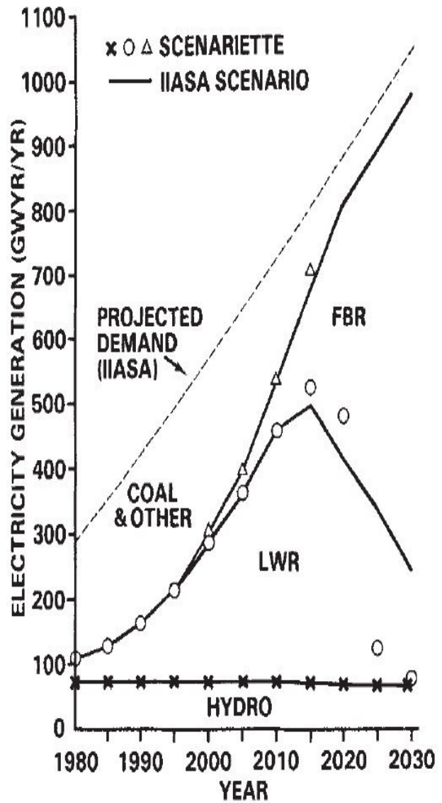
Fig. 3 Hydroelectric and nuclear power projections (for Western Europe, Japan, Australia and New Zealand). Points are derived from inputs to IIASA models (Fig. 1); curves are outputs. Rapid displacement of LWRs by FBRs is due to 2% cost difference (see Fig. 4).
