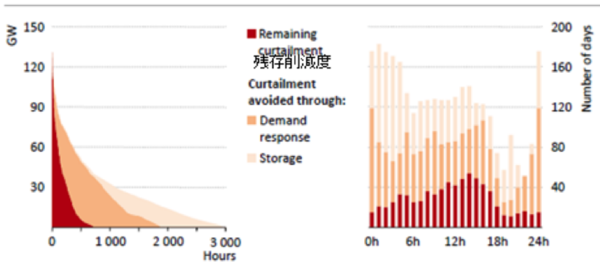
Demand-side response and storage technologies cut curtailment by around three-quarters in volume and number of hours
