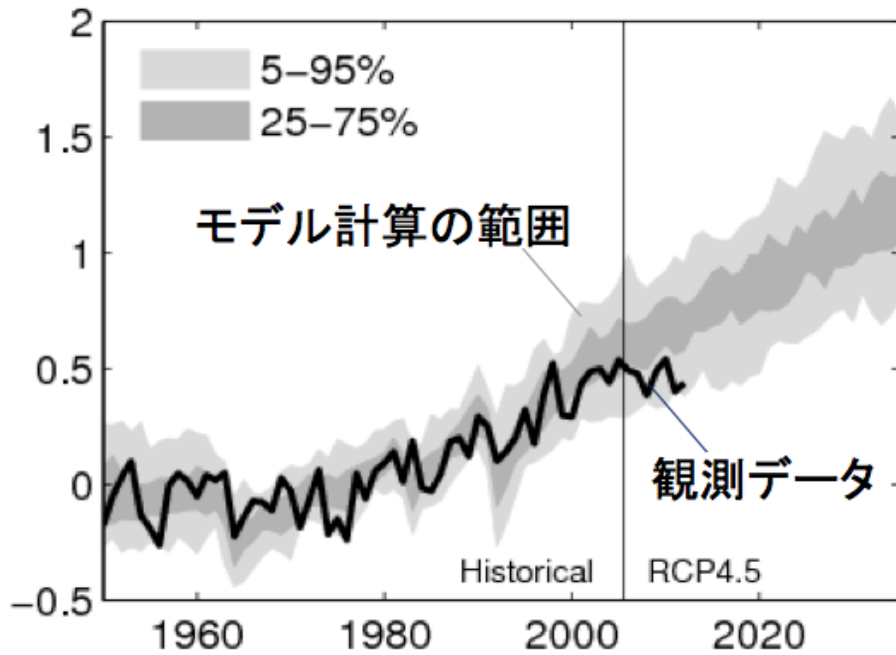
MASKED CMIP5 and HadCRUT4
